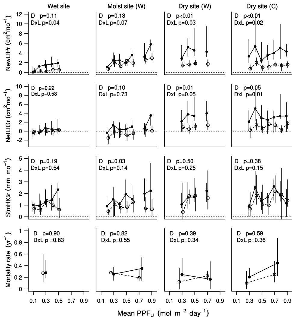
Fig. 4 Comparison of the performance of wet- ( filled circle ) versus dry- ( open circle ) distribution species grown at different understory light levels in wet, moist and dry sites , with ( W ) and without water supplementation ( C ). The symbols represent the medians, and vertical bars represent the inter-quartile range for each group of species at each light category. To improve legibility, plots with similar light levels were combined by averaging seedling performance within species. For mortality rates, we used only two light categories: less than and more than 0.5 \text{ mol m}^{-2} \text{ day}^{-1} . Only data for uncaged seedlings are reported. The P values in the panels represent the significance of the main effect of distribution on seedling performance ( D ) and the distribution \times light interaction ( D \times L ), using linear mixed-effect models for the growth variables and Cox models for mortality
